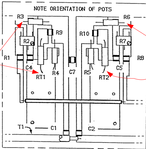
HB AMPLIFIER SINGLE STAGE: OUTPUT COMPONENTS (from 40D1468)
